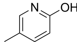
5-methylpyridin-2-ol
