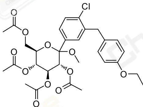
HY-329_3 Molecular Weight: 607.05
