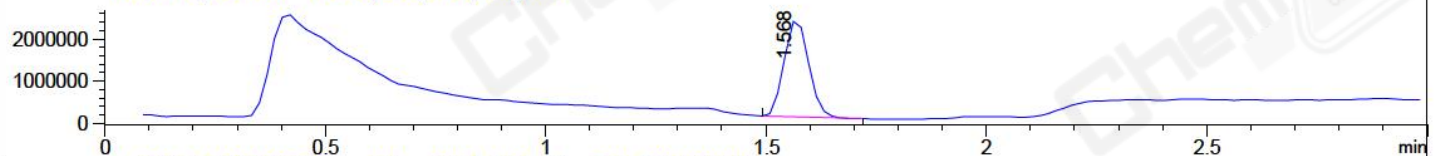
Ion 559.1, MSD1 559.1, Target Mass 558.1 +H Positive, EIC=558.8:559.8
