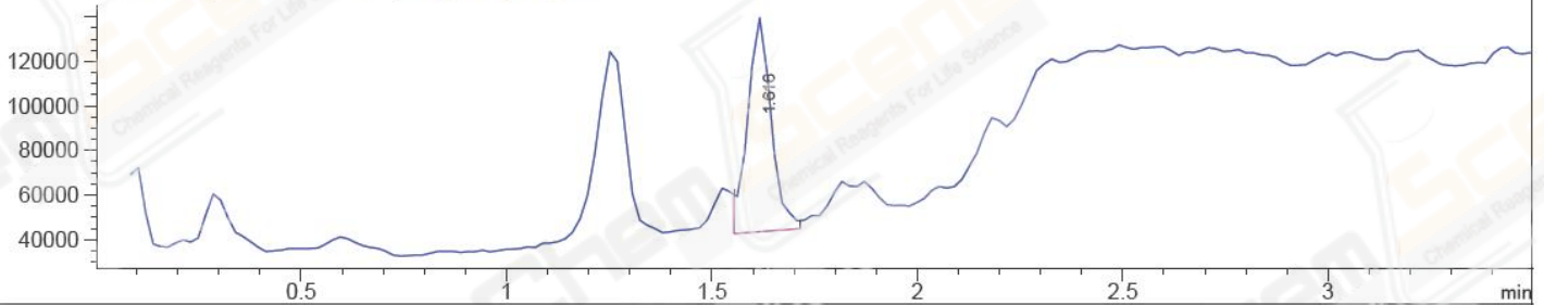
Ion 0, MSD1 0, Target Mass 0 Positive, EIC=-0.30:0.70
