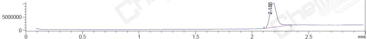
Ion 407.2, MSD1 407.2, Target Mass 407.2 Positive, EIC=406.9:407.9
