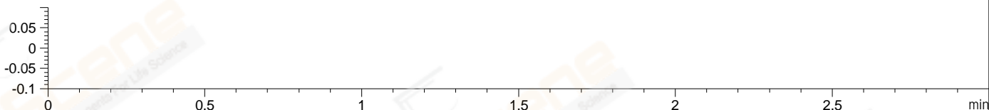
Ion 1, MSD1 1, Target Mass 0 +H Positive, EIC=0.7:1.7
