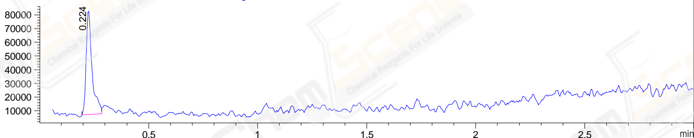
Ion 139, MSD1 139, Target Mass 138 +H Positive, EIC=138.7:139.7
