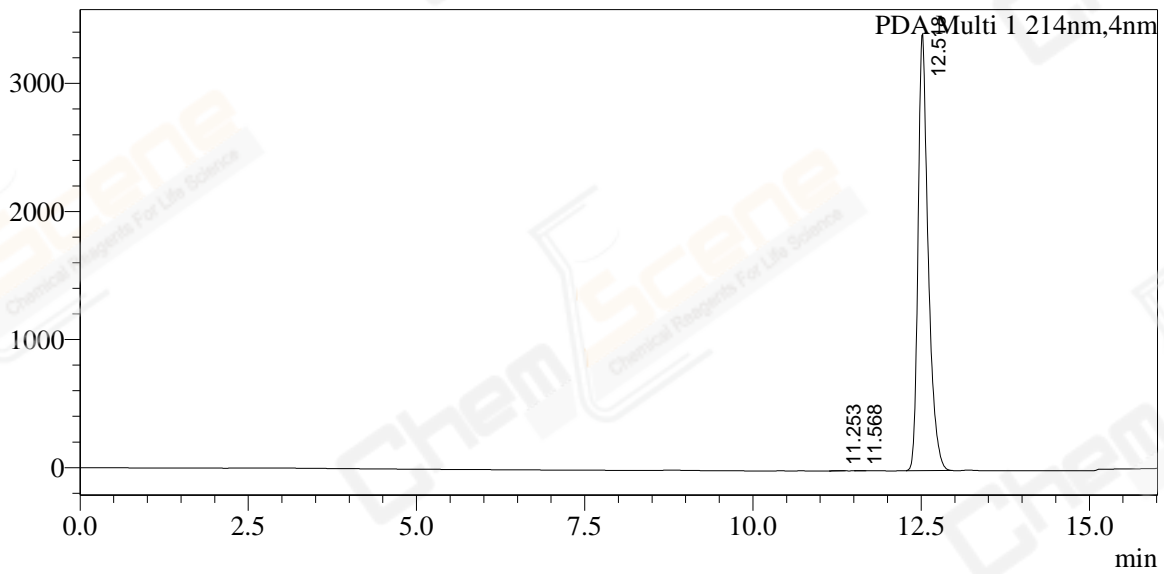
PDA Chromatogram
